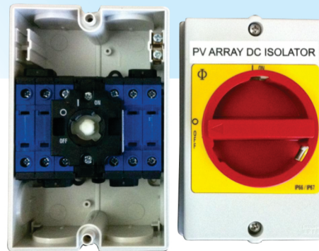
STANDARD ENCLOSURE 132H x 85W x 64D Order Code: KN909
