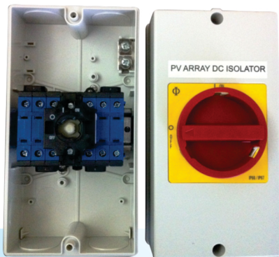
LARGE ENCLOSURE 178H x 100W x 93D Order Code: KN910
