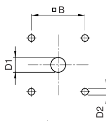
Mounting Holes
